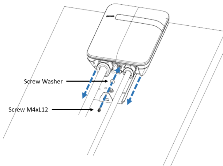
Figure 2-9 Screw locking position
