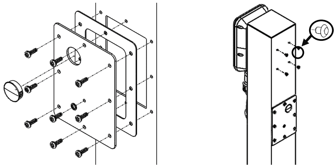
Fig. 8: Single EVSE Installation
