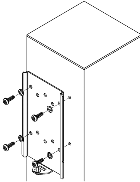
Fig 10: Install Mounting Bracket (Tighten to 13 inch-pounds)
