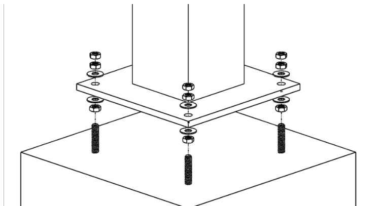
Fig. 4: Recommended Washer and Nut configuration
