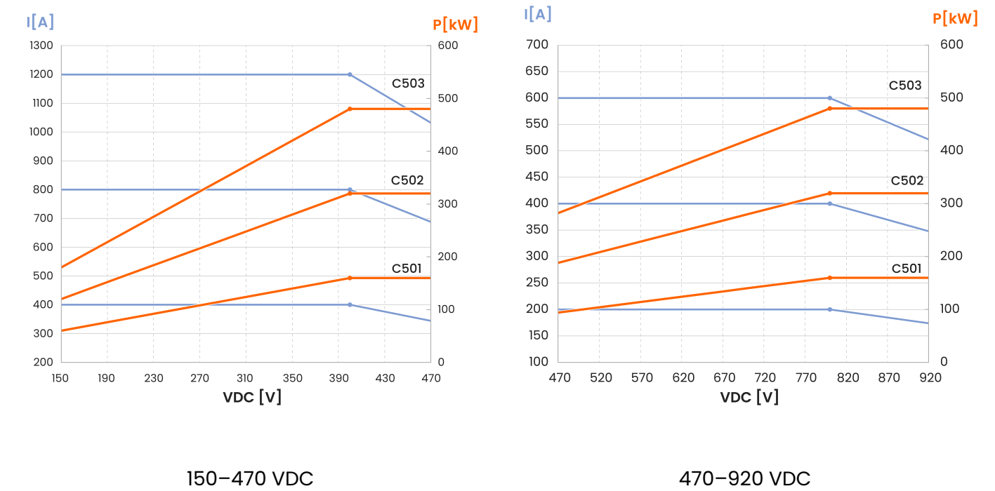
Power curve – continuous operation
