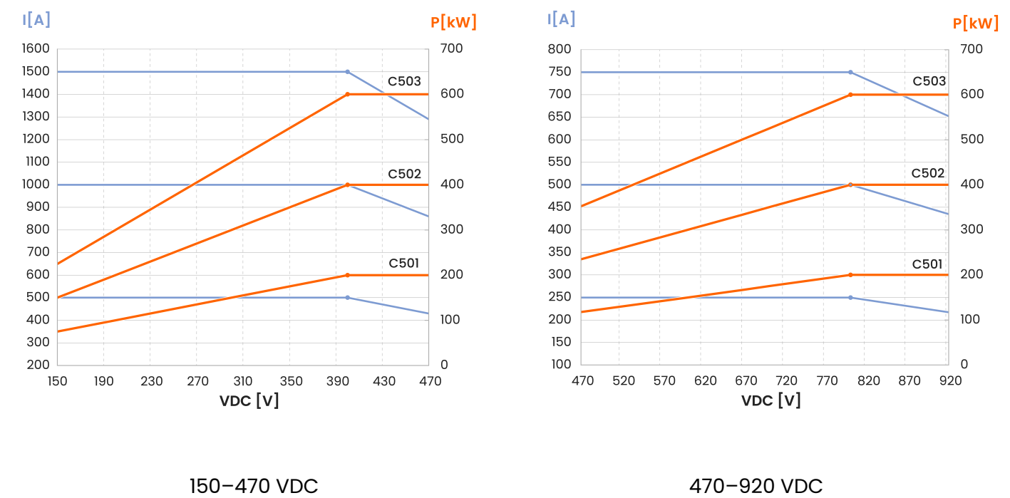
Power curve – standard operation
